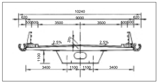
2. Open Box Girder
