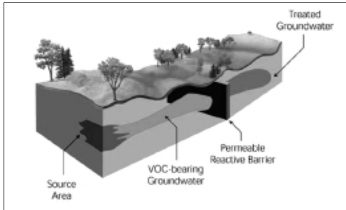
1. (PRBs)
